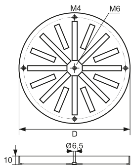
Installation with 1 screw (1xM6) Installation with 5 screws (1xM6+4xM4) only for diffuser size 800
