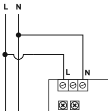
series SILENTA-ST, SILENTA-STH
