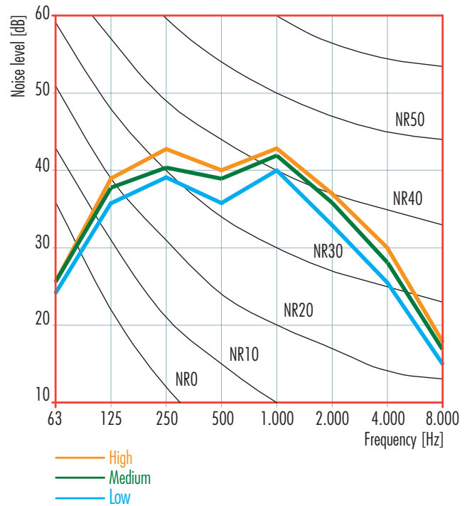
Sound curve
