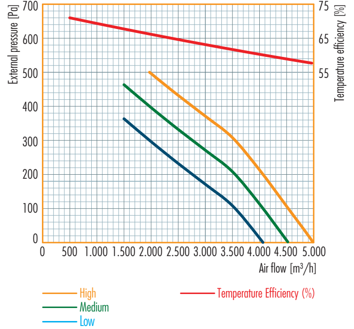
Performance curve
