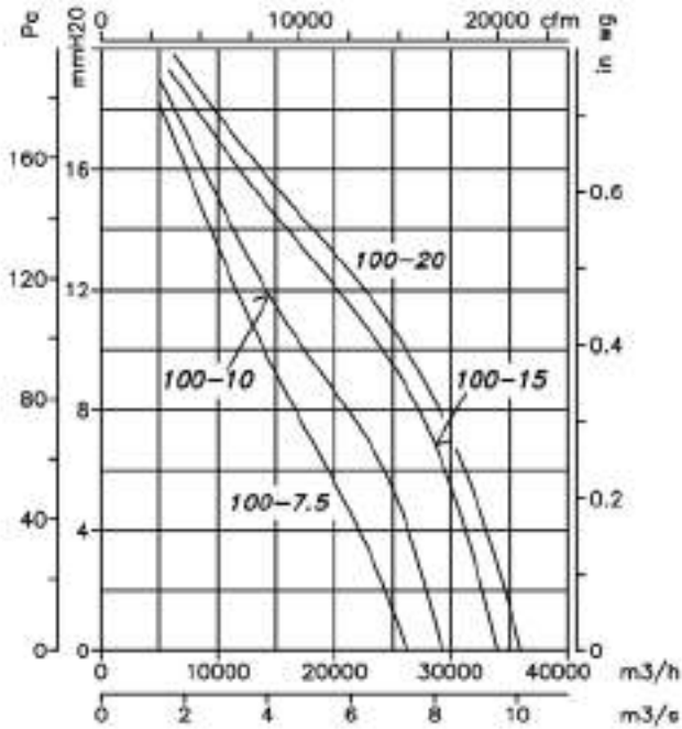
8 poles (2-speed 4/8 motor)
