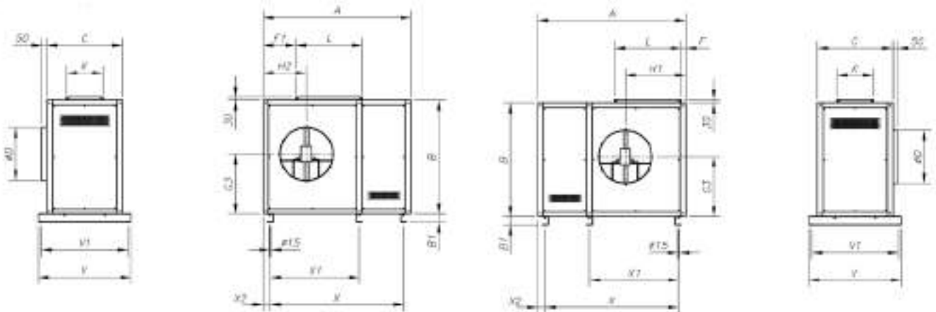
Vertical impulsion on request (V) RD 0
