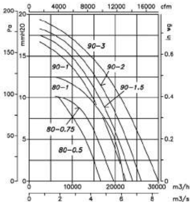
8-Pole=900 r/min
