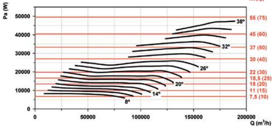
Absorbed power
