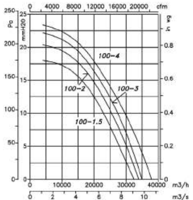
8-Pole=900 r/min
