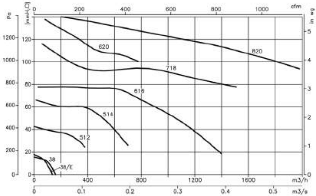
2T/2M=3600 r/min
