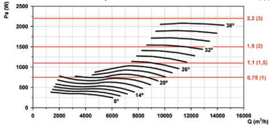
Absorbed power
