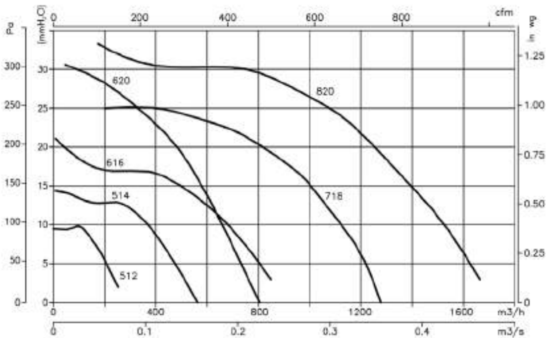
4T/4M=1800 r/min
