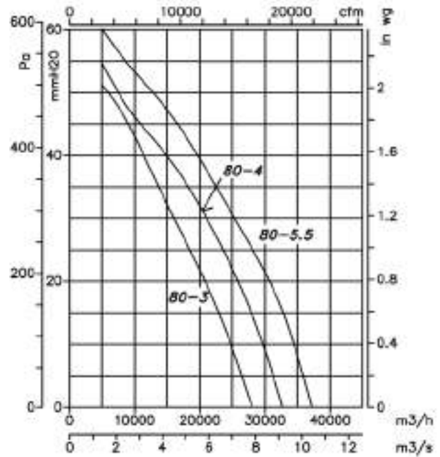
4-Pole=1800 r/min
