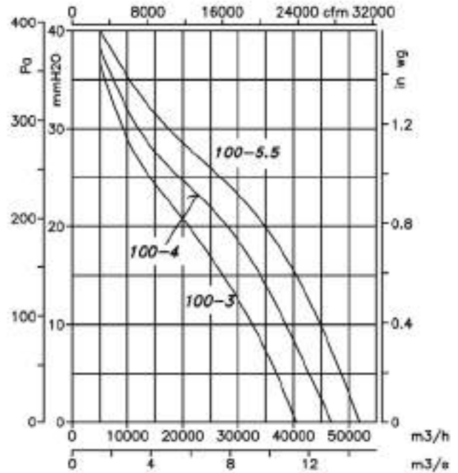
6-Pole=1200 r/min
