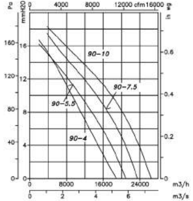
8 poles (2-speed 4/8 motor)
