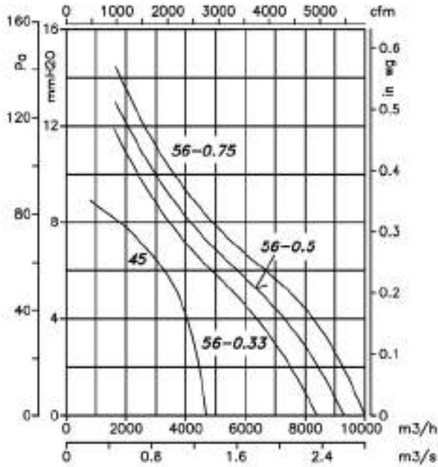
6-Pole=1200 r/min
