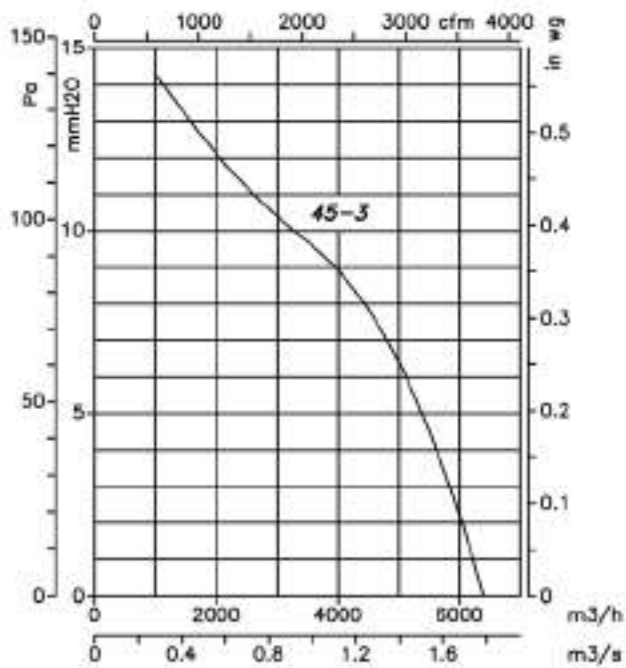
4 poles (2-speed 2/4 motor)
