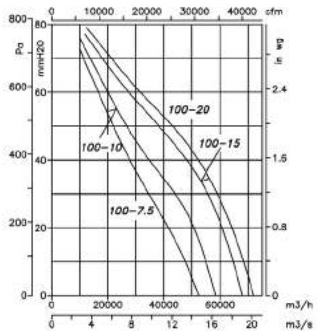
4-Pole=1800 r/min
