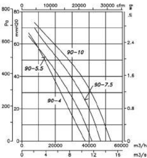
4-Pole=1800 r/min
