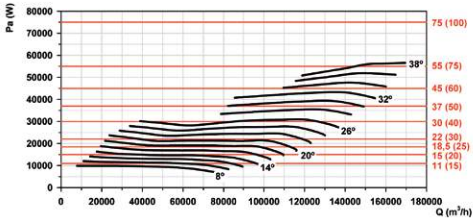
Absorbed power
