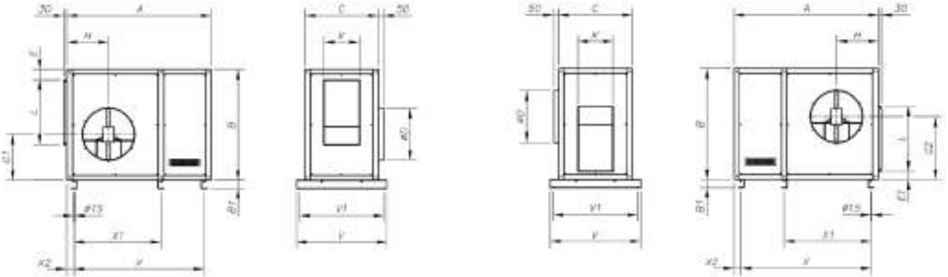
Vertical impulsion on request (V) RD 0
