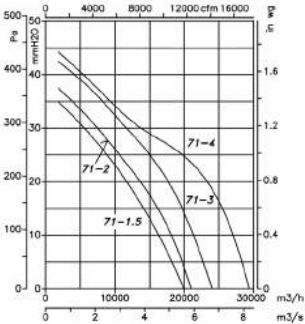
4-Pole=1800 r/min
