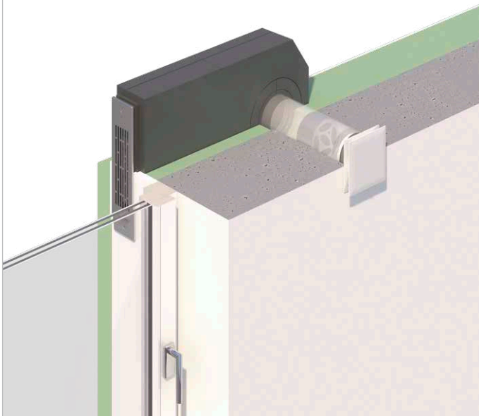
ZLA LE – Installation example DN 100 mm
