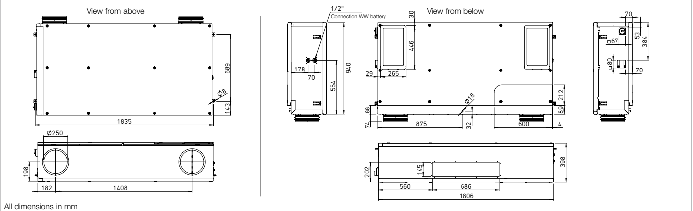
All dimensions in mm
