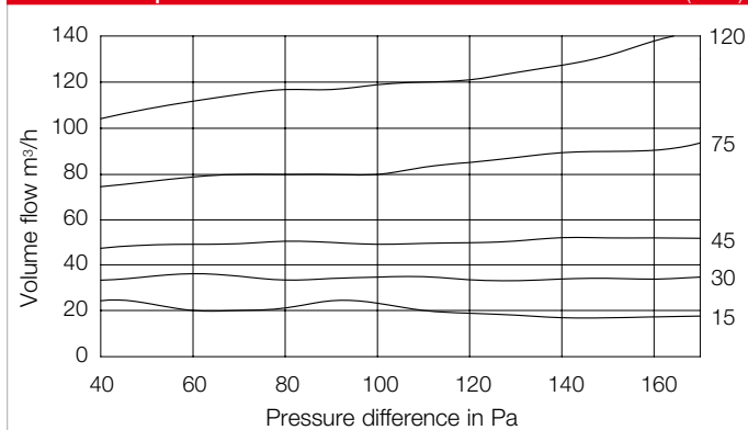
Volume flow performance curves AE GB Nominal volume flow (m³/h)
