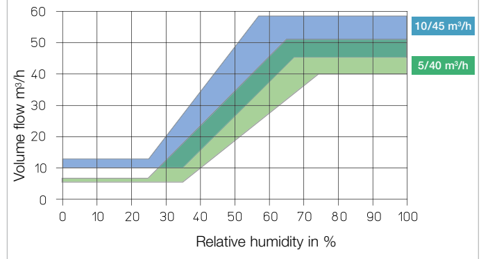
Operating range AE Hygro
