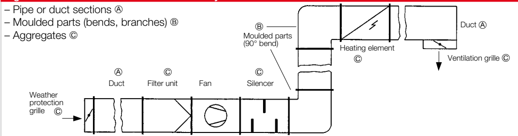
Figure 9 Pressure losses in a ventilation system
