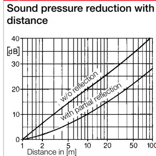
Figure 5 Sound pressure reduction with distance
