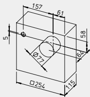
ELS-surface-mounted unit
