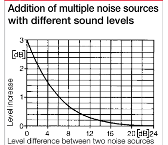
Figure 7 Addition of multiple noise sources with different sound levels
