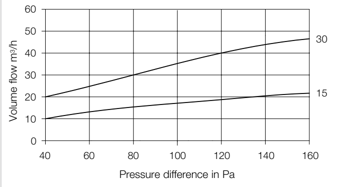
Volume flow performance curve AE B Nominal volume flow (m 3 /h)
