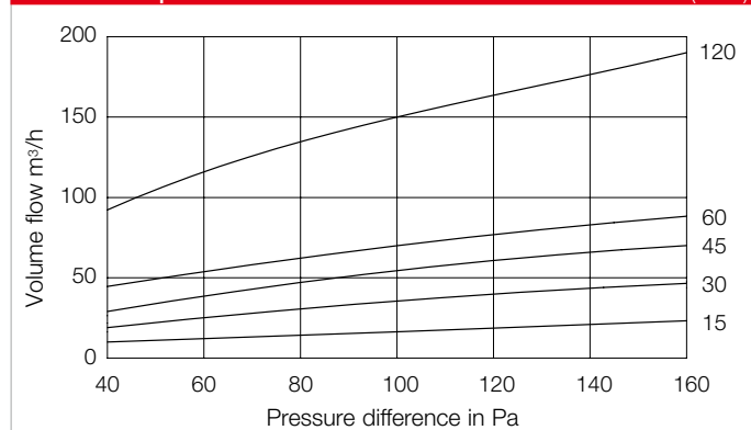
Volume flow performance curves AE GBE Nom. volume flow (m³/h)
